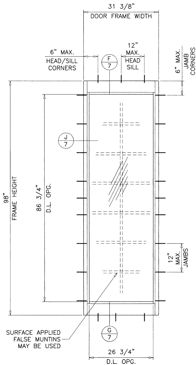
TYPICAL ELEVATION ( O )
