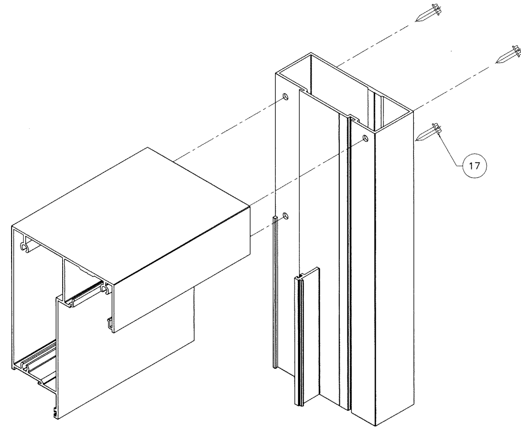
SIDELITE FRAME CORNER
