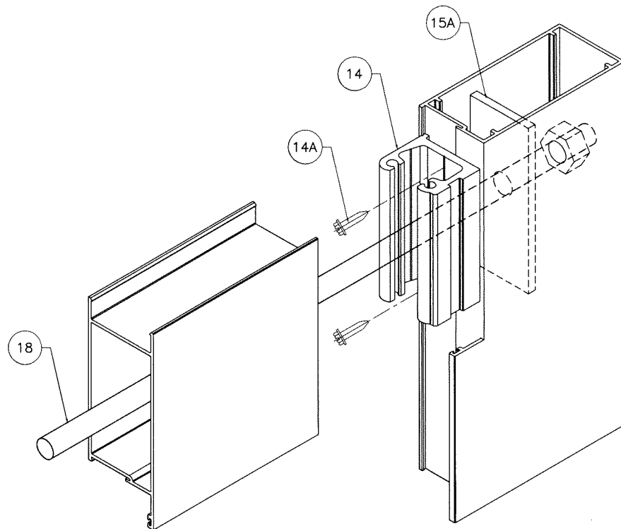
LEAF CORNER
