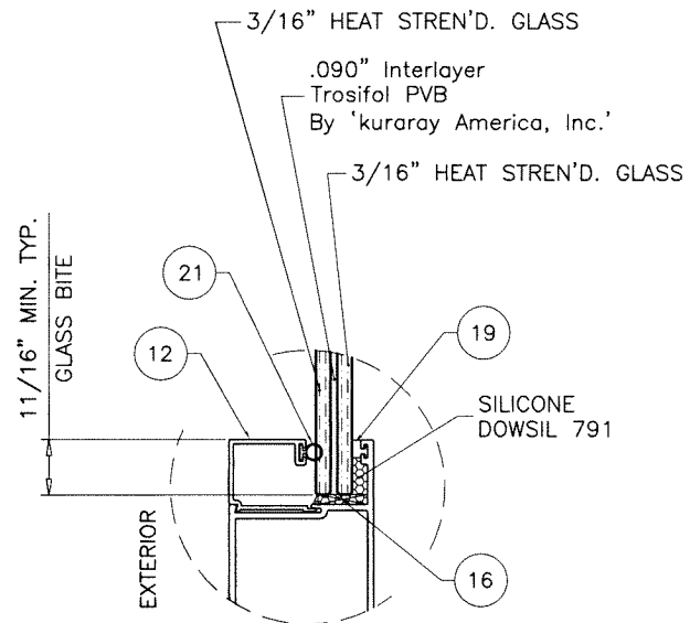
GLAZING DETAIL
